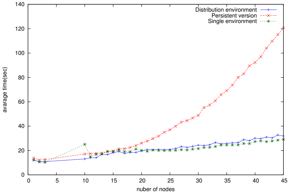
write benchmark
