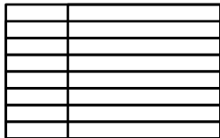
Key-Value
