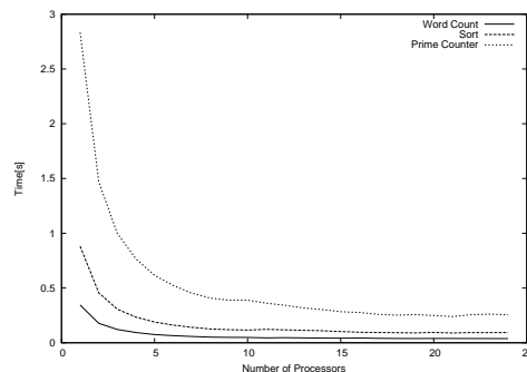
図 1 Execution time
