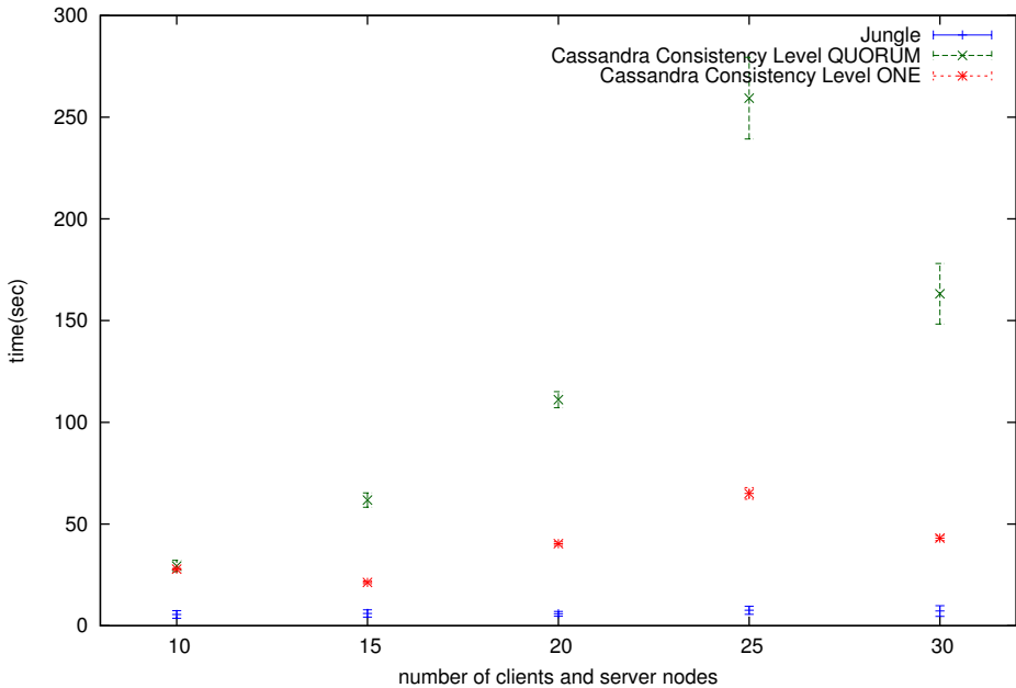
distributed write benchmark (Requests : clients * 20,000)
