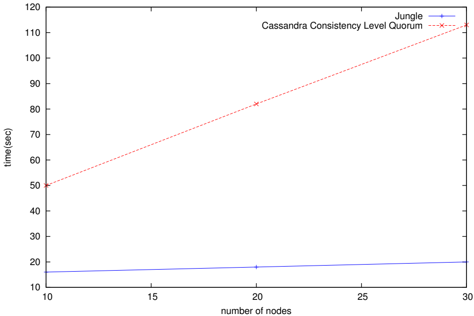
write benchmark (Requests : clients * 50,000)
