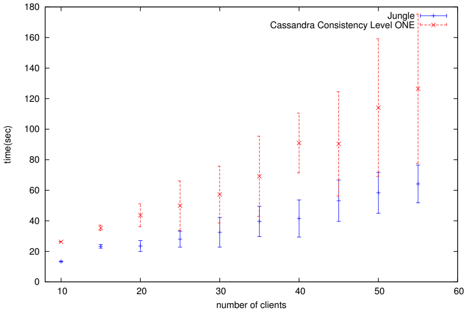
Single node write benchmark (Requests : clients * 20,000)
