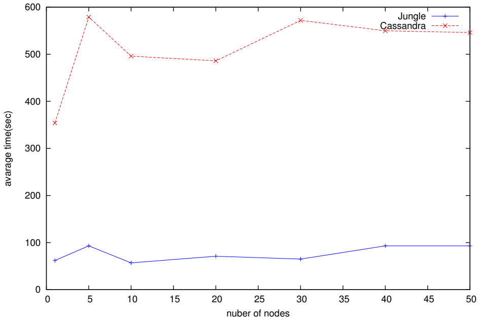
write benchmark
