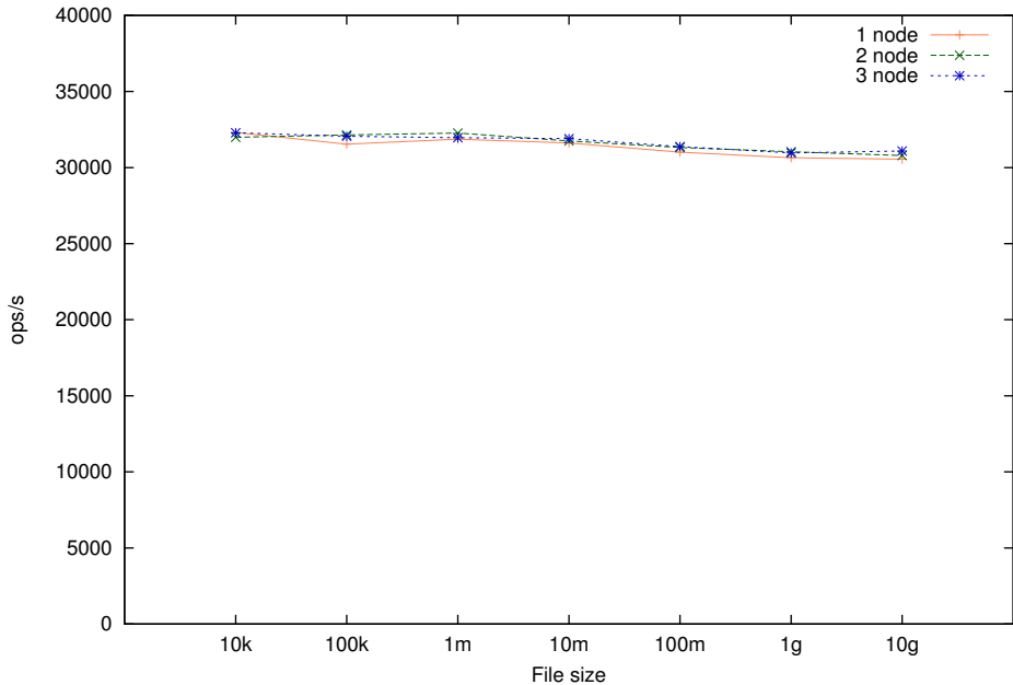
GFS2 3 node read benchmark
