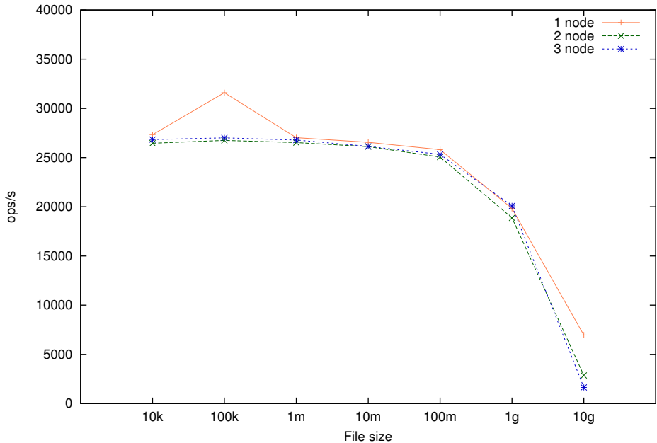
GFS2 3 node write benchmark
