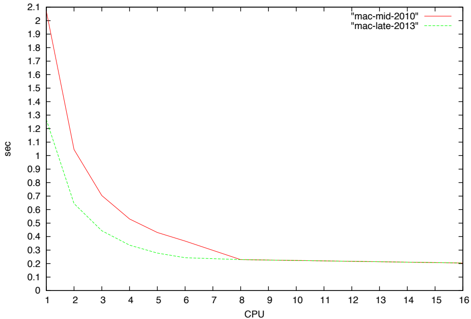
Sort Benchmark
