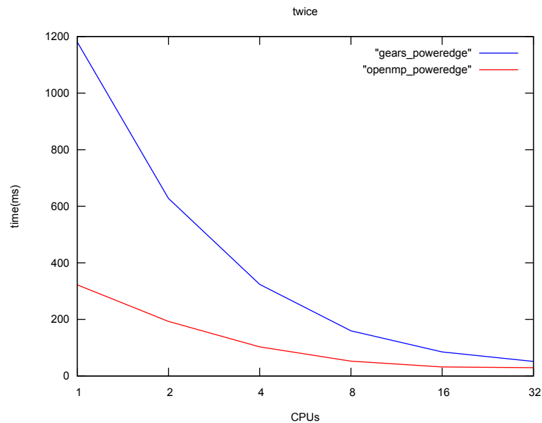
図 6.4: vs OpenMP
