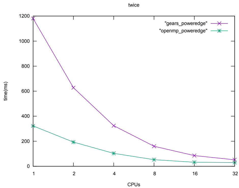
図 6.4: vs OpenMP
